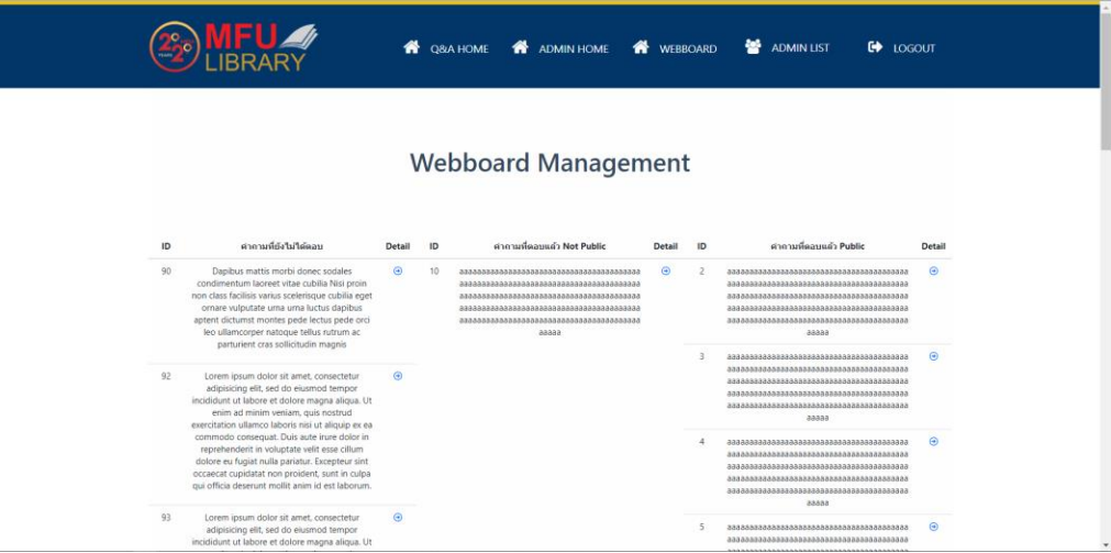
Figure 4.7 Webboard management
