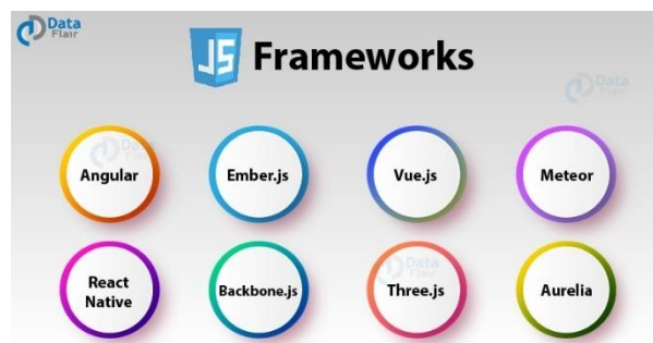
Figure 2.2 Framework
