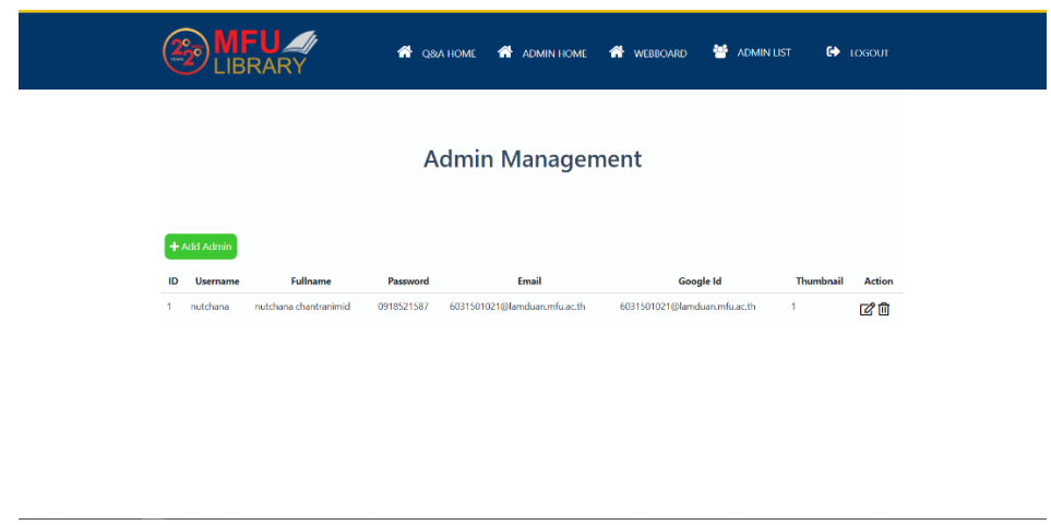
Figure 4.4 Admin page
