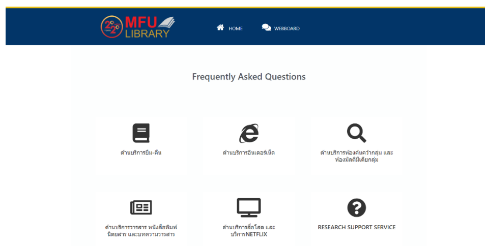
Figure 4.1 Home page
