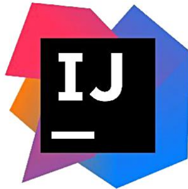
Figure 2.2 IntelliJ
