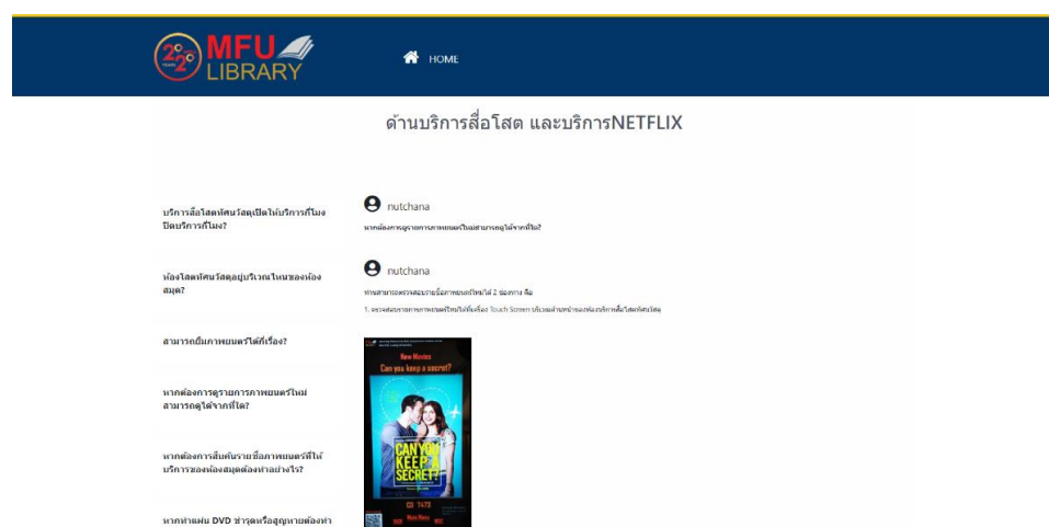
Figure 4.2 Details page
