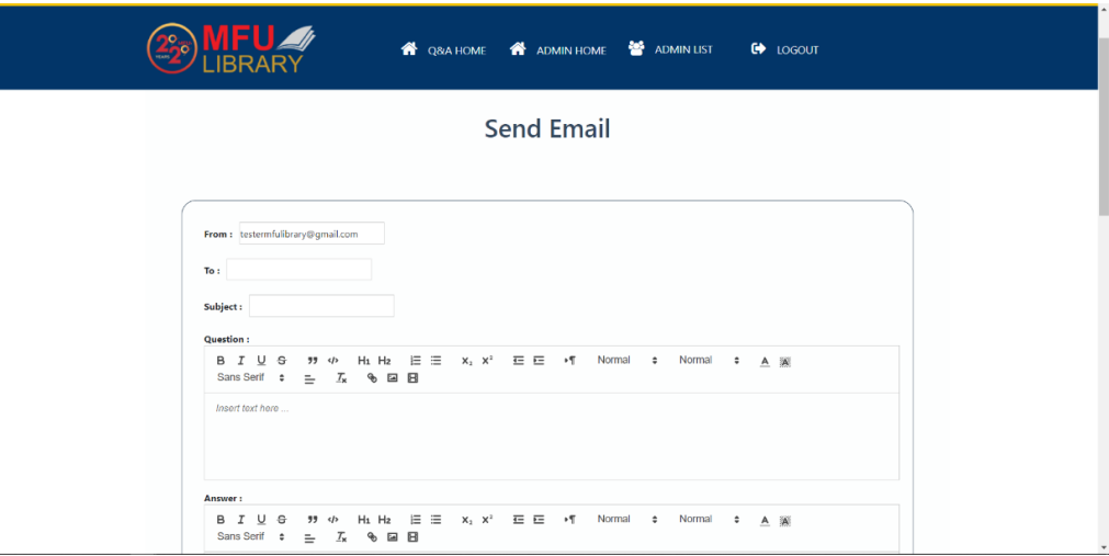
Figure 4.8 Send Email
